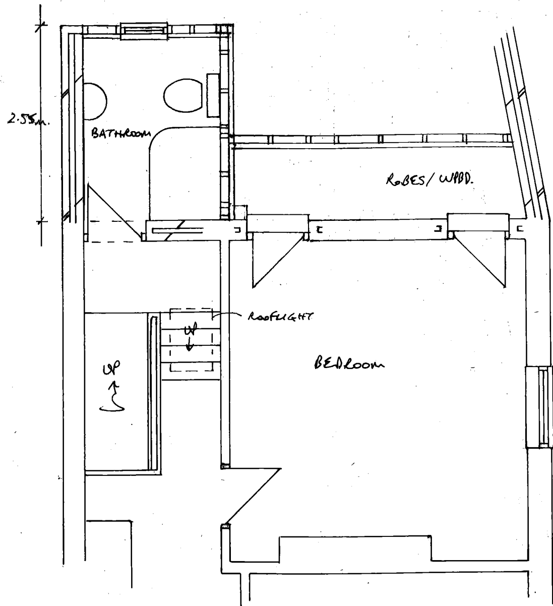
PROPOSED 2ND FLOOR 1:50
