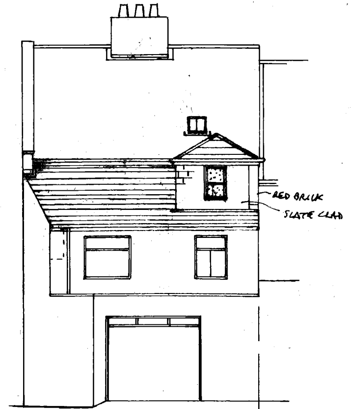
PROPOSED REAR 1:100
